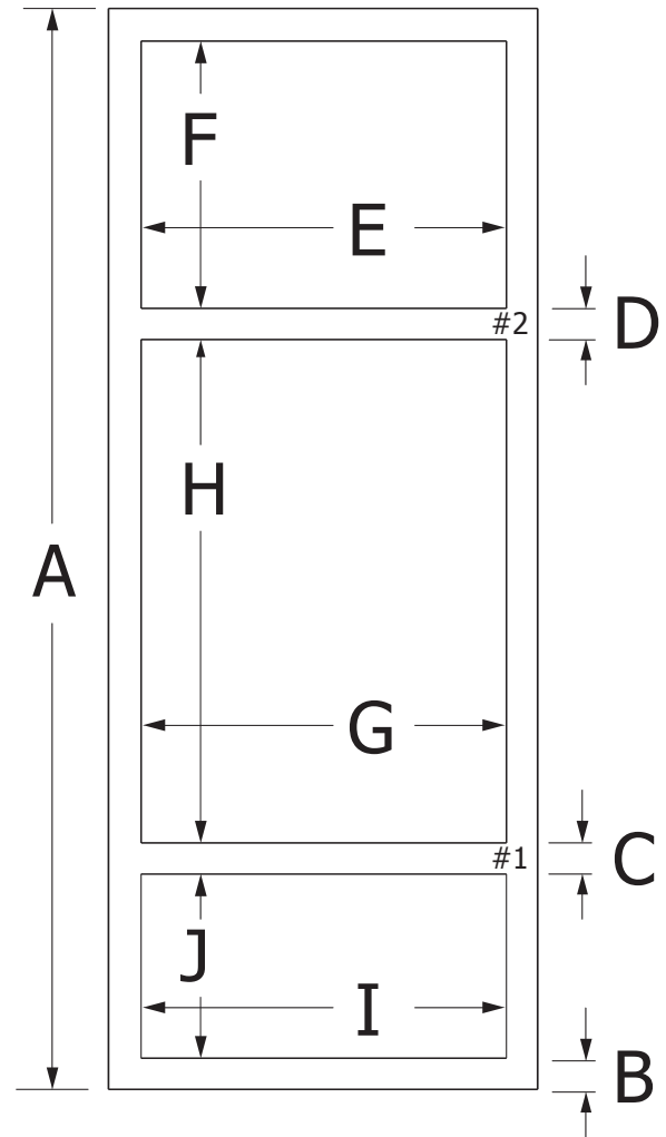
MICROWAVE / WALL OVEN / WARMING DRAWER FRAME
