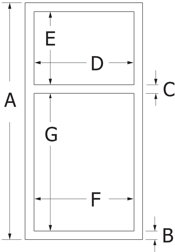
MICROWAVE / WALL OVEN FRAME
